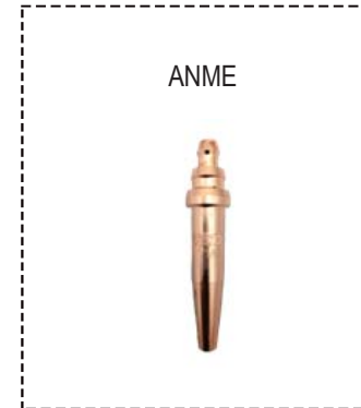
CUTIING NOZZLE ANME: 1/16, 1/64, 1/32, 3/32 , 3/64, 5/64
