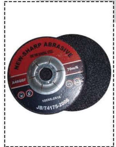
Cutting/grinding disc, flexible 4"x2.5/3.0x16
