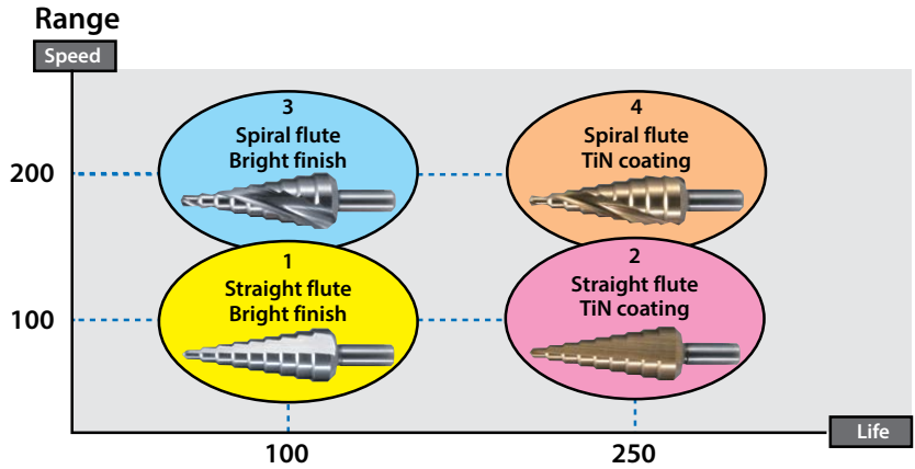
Material chart
